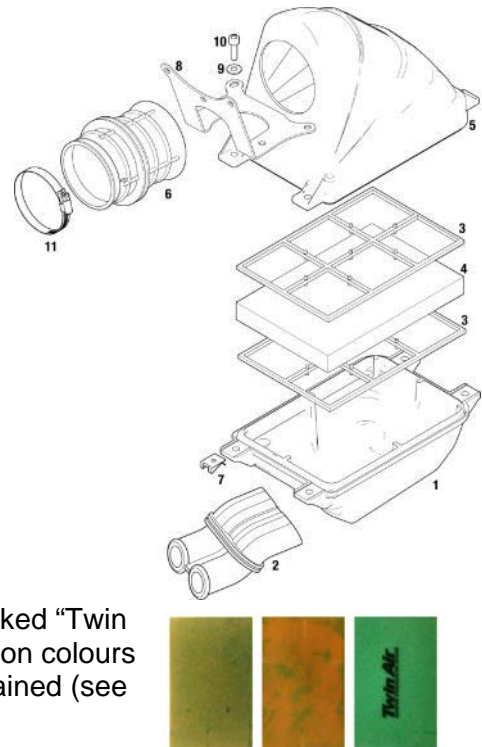
Pos. 4, legal air filter executions
